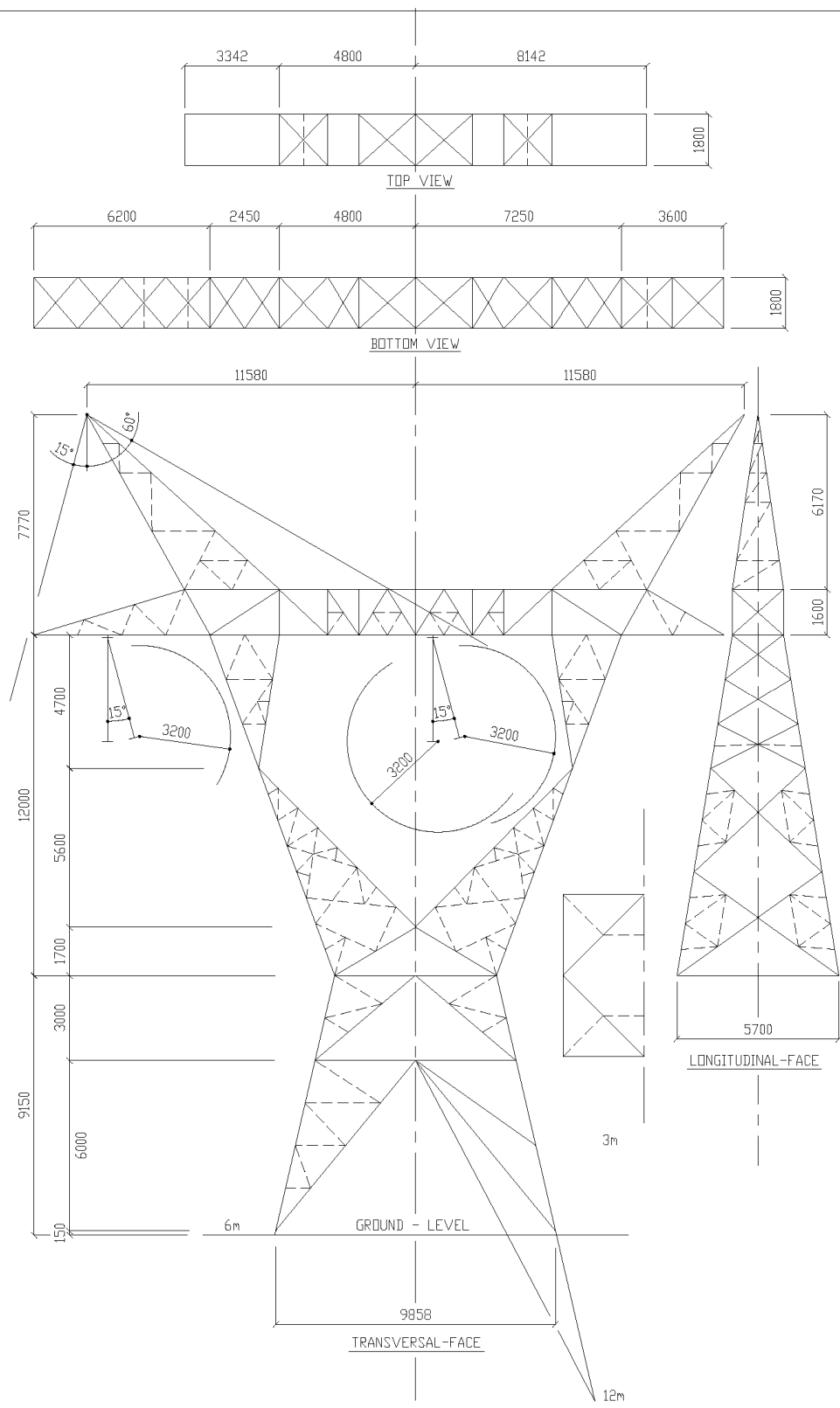
400 kV TRANSMISSION LINE 35°-60° A/S & 0° TERM. WITH 0°-45° CLOSING SPAN TOWER TYPE "517F"
